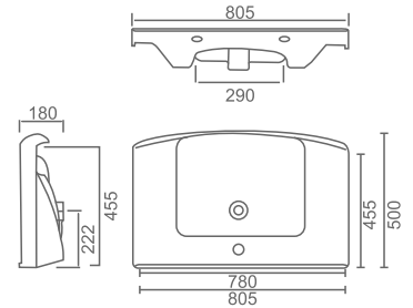
5706 Cabinet Washbasin 80 cm.
