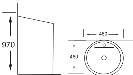
IC 021 Pedestal Basin 450x460x970 mm
