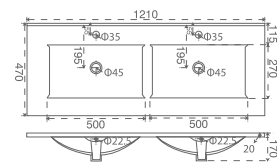
IYS27293 - 120D Slim Cabinet Washbasin 120 cm
