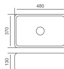
I059-S Above Counter Mounting 480x370x130 mm
