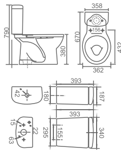
3623 Closet S-Trap (With Out Hole)
