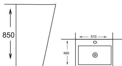
IC 001 Pedestal Basin 510x460x850 mm
