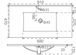
IYS27293 - 90 Slim Cabinet Washbasin 90 cm
