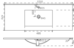
IYS27286 – 120 Slim Cabinet Washbasin 120 cm
