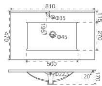
IYS27293 - 80 Slim Cabinet Washbasin 80 cm
