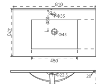
IYS27286 – 80 Slim Cabinet Washbasin 80 cm
