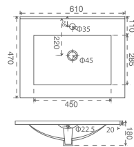
IYS27286 – 60 Slim Cabinet Washbasin 60 cm
