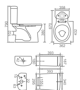
3633 Closet P-Trap (With Out Hole)
