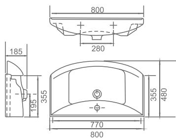
5702 Cabinet Washbasin 80 cm
