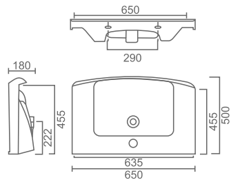
5707 Cabinet Washbasin 65 cm.
