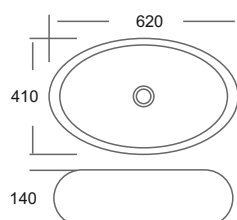
IH-425-G04 Above Counter Mounting 620x410x140 mm
