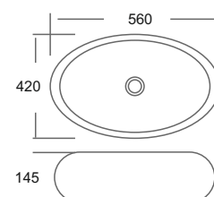
IH-253-27G Above Counter Mounting 560x420x145 mm
