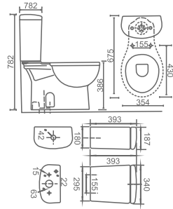
3523 Closet S-Trap (With Out Hole)
