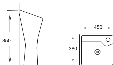
IC 019 Pedestal Basin 450x380x850 mm
