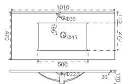
IYS27293 - 100 Slim Cabinet Washbasin 100 cm
