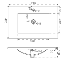
IYS27286 – 70 Slim Cabinet Washbasin 70 cm
