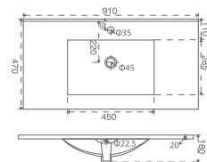
IYS27286 – 90 Slim Cabinet Washbasin 90 cm
