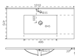
IYS27286 – 100 Slim Cabinet Washbasin 100 cm
