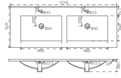
IYS27286 – 120D Slim Cabinet Washbasin 120 cm
