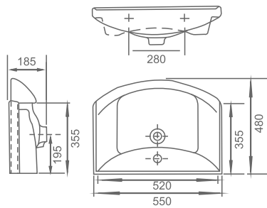
5704 Cabinet Washbasin 55 cm
