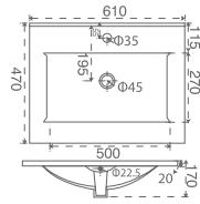
IYS27293 - 60 Slim Cabinet Washbasin 60 cm
