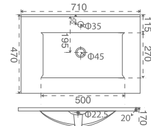
IYS27293 - 70 Slim Cabinet Washbasin 70 cm
